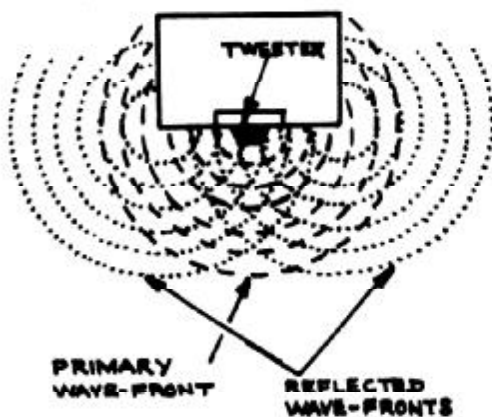
CONVENTIONAL LOUSPEAKER SYSTEM SHOWING REFLECTED WAVES FROM CABINET EDGES.
